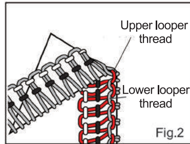
Low tension of lower looper or high tension of upper looper thread
